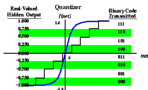
Fig.4: The Quantization of Hidden Unit Outputs
