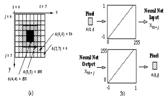
Fig.5: The Pixel-to-Real and Real-to-Pixel Conversions
