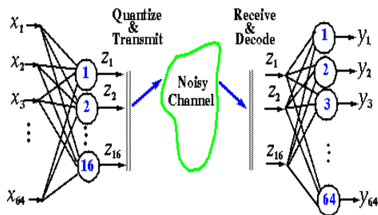
Fig.3: The Image Compression Scheme using the Trained Neural Net
