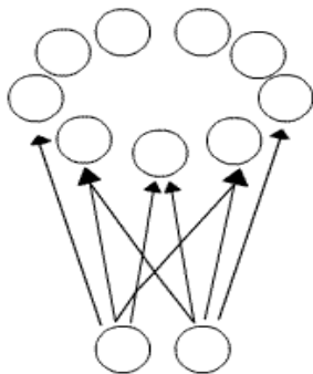
Fig.9: Kohonen net
