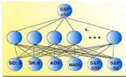
Fig.6: Neural Network
