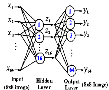
Fig.2: Bottleneck-type Neural Net Architecture for Image Compression
